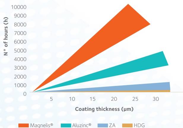
Corrosion resistance by salt spray test (average):
