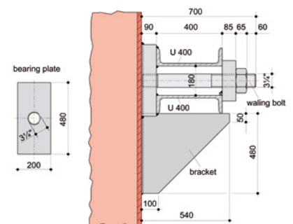
Solutions for execution details
