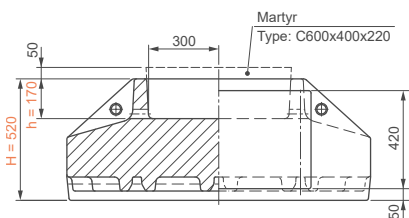
Coupe 1-1 (UZD 14-28) [mm]
