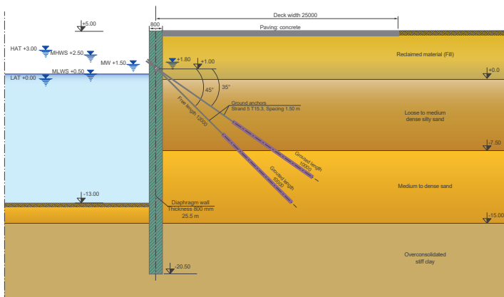
Figure 1. Cross section of the cruise ship terminal with steel sheet piles and with a diaphragm wall (design by Tractebel Engineering).
